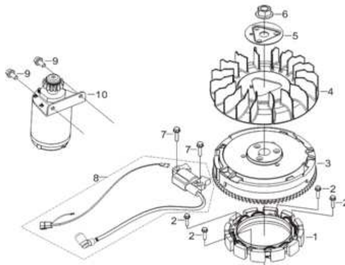
FIG.8 FLYWHEEL / IMPELLER / STARTER PULLEY / IGNITION COIL
