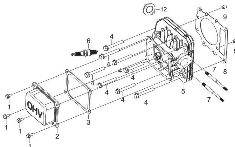
FIG.3 HEAD SUBASSEMBLY, CYLINDER / PLUG,SPARK
