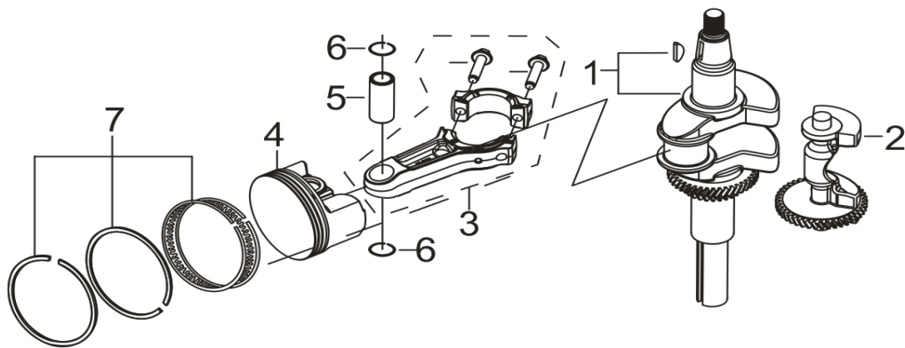
FIG.4 ROD,CRANKSHAFT CONNETING
